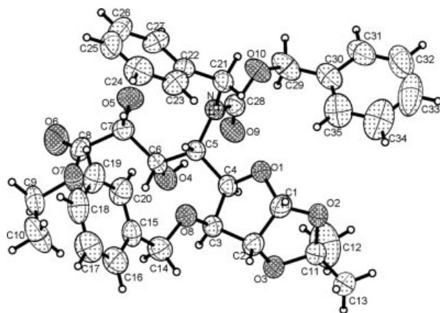
Figure 2. ORTEP diagram of the molecule 9a .
