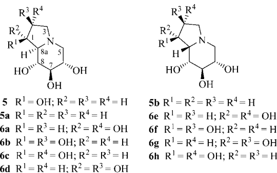
Figure 1. Indolizidine alkaloids.
