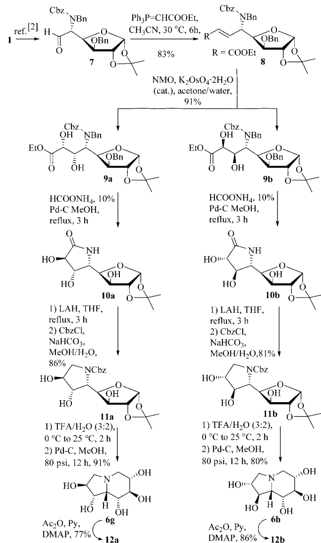
Scheme 2. Synthesis of indolizidine alkaloids 6g and 6h .
