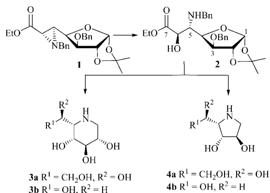
Scheme 1. Piperidine and pyrrolidine alkaloids.
