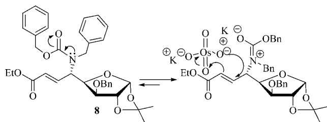
Figure 3. Plausible transition state for the observed selectivity.
