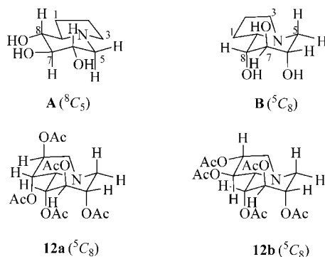
Figure 4. Conformations of indolizidines.
